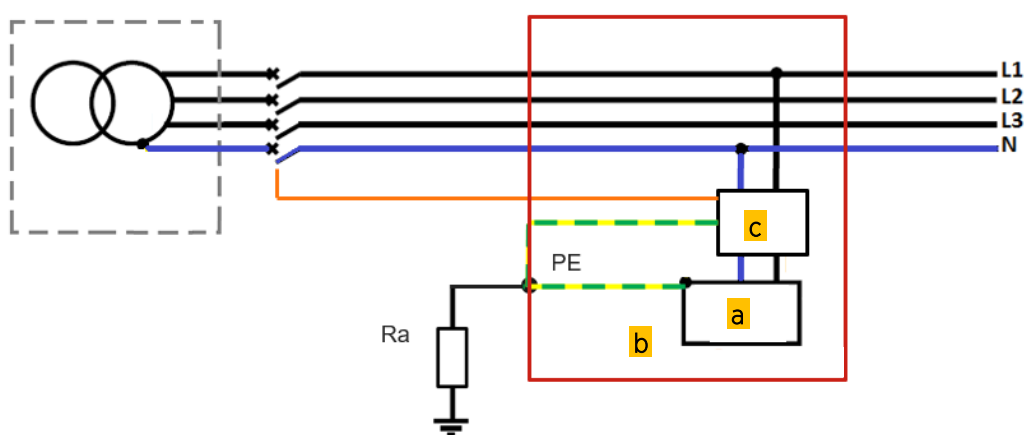
Figure 3: IT Scheme
