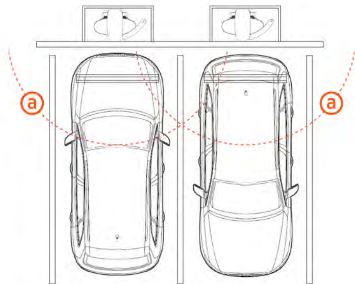
(a) Cable reach radius: 3.76 m (12 ft 4 in)
